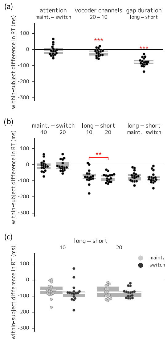
FIG. 7. (Color online) Box-and-swarm plots of between-condition differences in reaction time for experiment 2. Boxes show first and third quartiles and median values; individual data points correspond to each listener; asterisks indicate comparisons with corresponding coefficients in the statistical model that were significantly different from zero. (a) Main effects of attention, spectral degradation, and gap duration (faster response time in trials with 20-channel vocoding, and in long-gap trials). (b) Two-way interactions (larger difference in reaction times between long- and short-gap trials in the 10- versus the 20-channel condition). (c) Three-way interaction (no statistically significant difference). *** = p < 0.001 .
